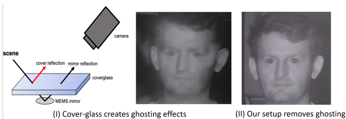
Fig. 3: The coverglass induces ghosting and double images. With a combination of using Brewster's angle, NIR notch filter and absorbing film, we eliminate the ghosting.
